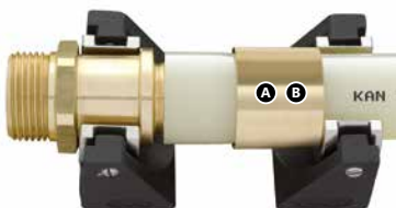
Installation of male and female pipe connectors \text{Ø}25 \times 3,5
