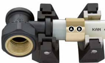
Installation of wallplate elbows PPSU
