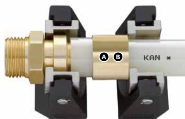
Installation of male and female pipe connectors \text{Ø}12 \times 2 , \text{Ø}14 \times 2 , \text{Ø}18 \times 2 , \text{Ø}18 \times 2,5
